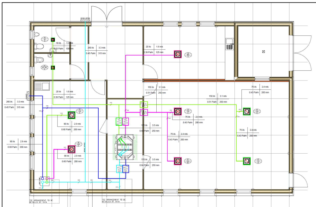
Figure 21: Ventilation Strategy Plan
