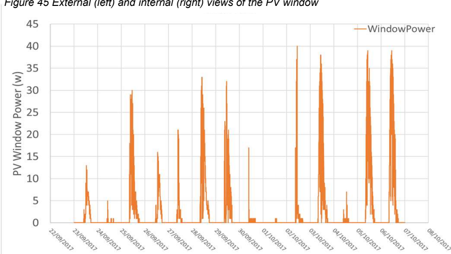
Figure 46 : Absolute power output of the Sunplus window during the test period
